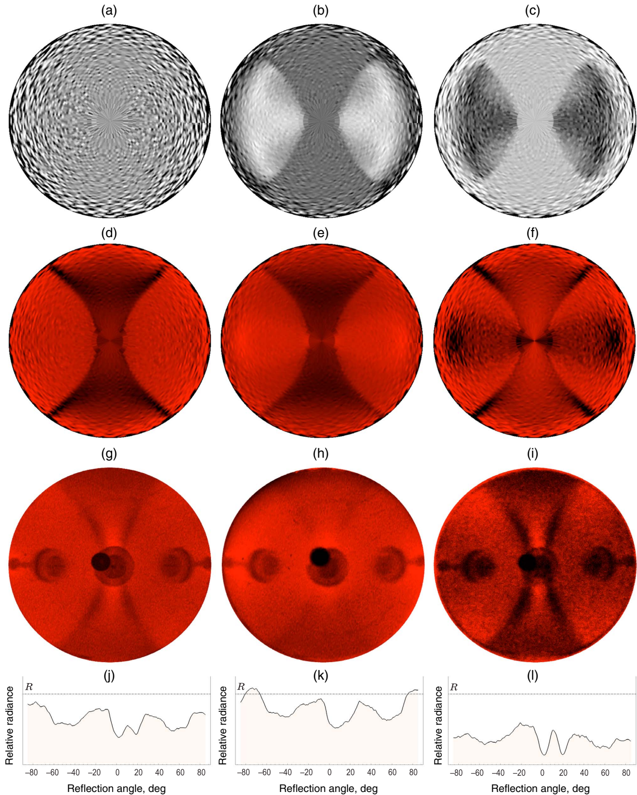
Fig. 3. Angular diagrams of the total radiance and of the polarization components of a diffuse light field scattered by the surfaces of the following diffraction gratings: (1) with ideal conduction (computer model, maximum deviation of the S and P components from the ideal Lambertian level 5%–6%); (2) with gold coating (computer model, excess of the ideal Lambertian level of the S component as much as 1.5%–2%); (3) with gold coating (actual experiment, excess of the ideal Lambertian level of the S component 1%–1.5% in the angular directions that correspond to the calculated maximum in the computer model).
