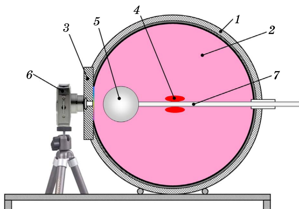
Fig. 1. Layout of an apparatus for studying the scattering of a diffuse light field by the surface of a diffraction grating.
