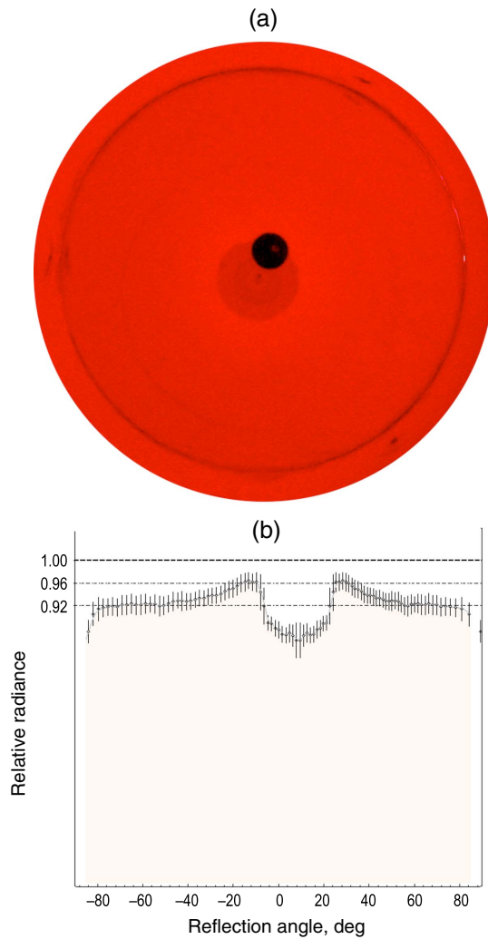
Fig. 2. For calculating the maximum possible radiance (for ideal Lambertian reflection) of some component of scattered radiation, using a gold mirror as an example.
