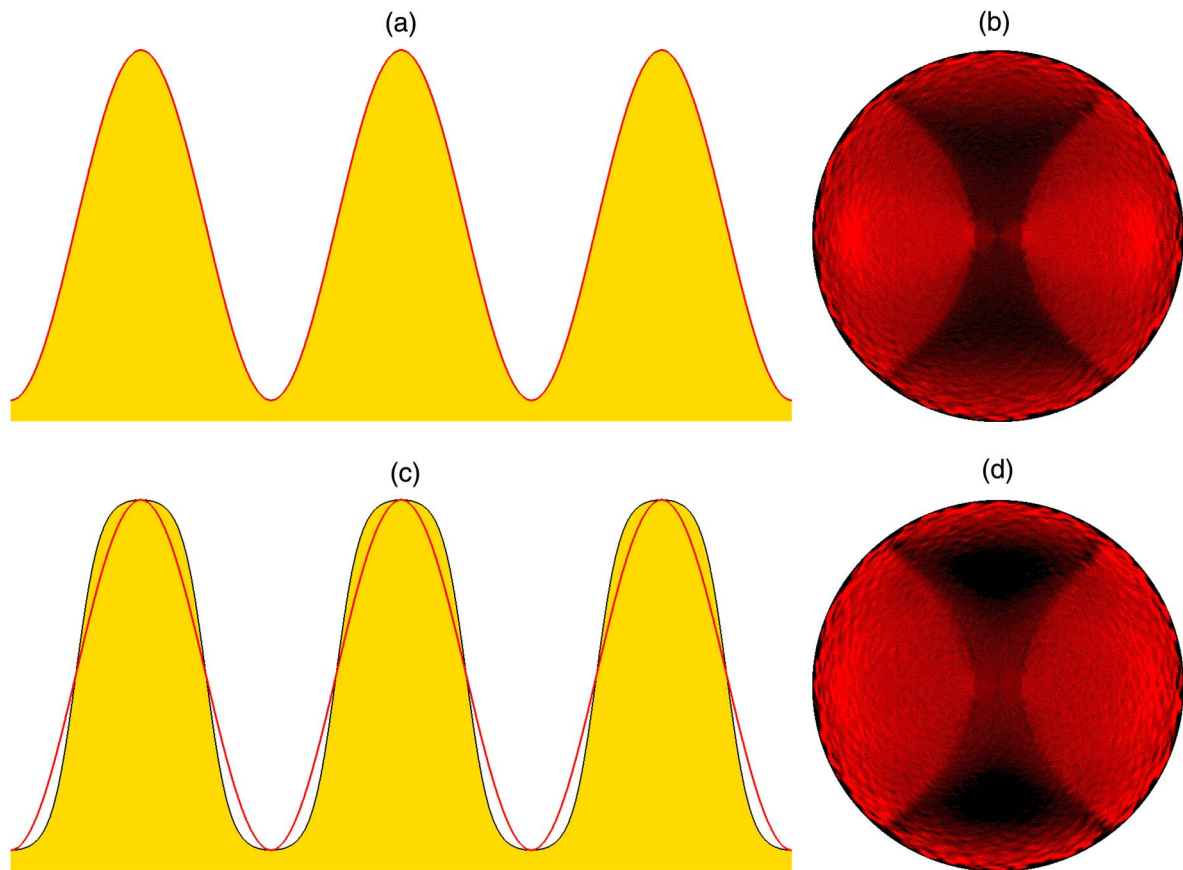
Fig. 4. Dependence of the manifestation of the predicted effect on the accuracy of the grating microrelief.
